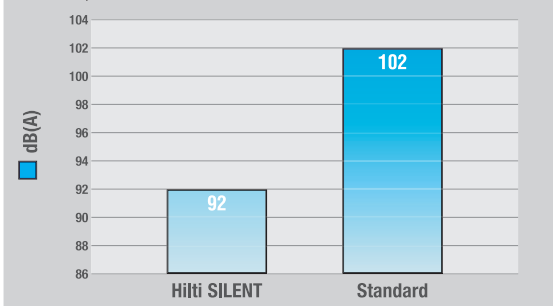
Noise measurements with DS-TS5-SE electric wall saw, reinforced concrete, 700 mm saw blade diameter
